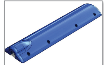
CAD rendering of a custom ScanMed coil cover to be used as an FDM mold master for creating a silicone mold.
