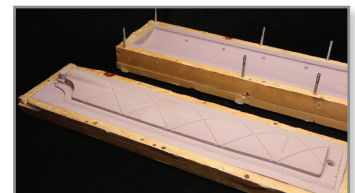
Silicone mold created using the FDM master pattern and used to produce cast urethane coil covers.
