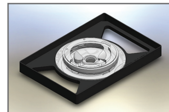
A 3D rendering of the assembled perfusion chamber in a microscope.
