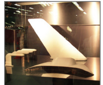
Antenna and other components being manufactured by a Fortus FDM machine.
